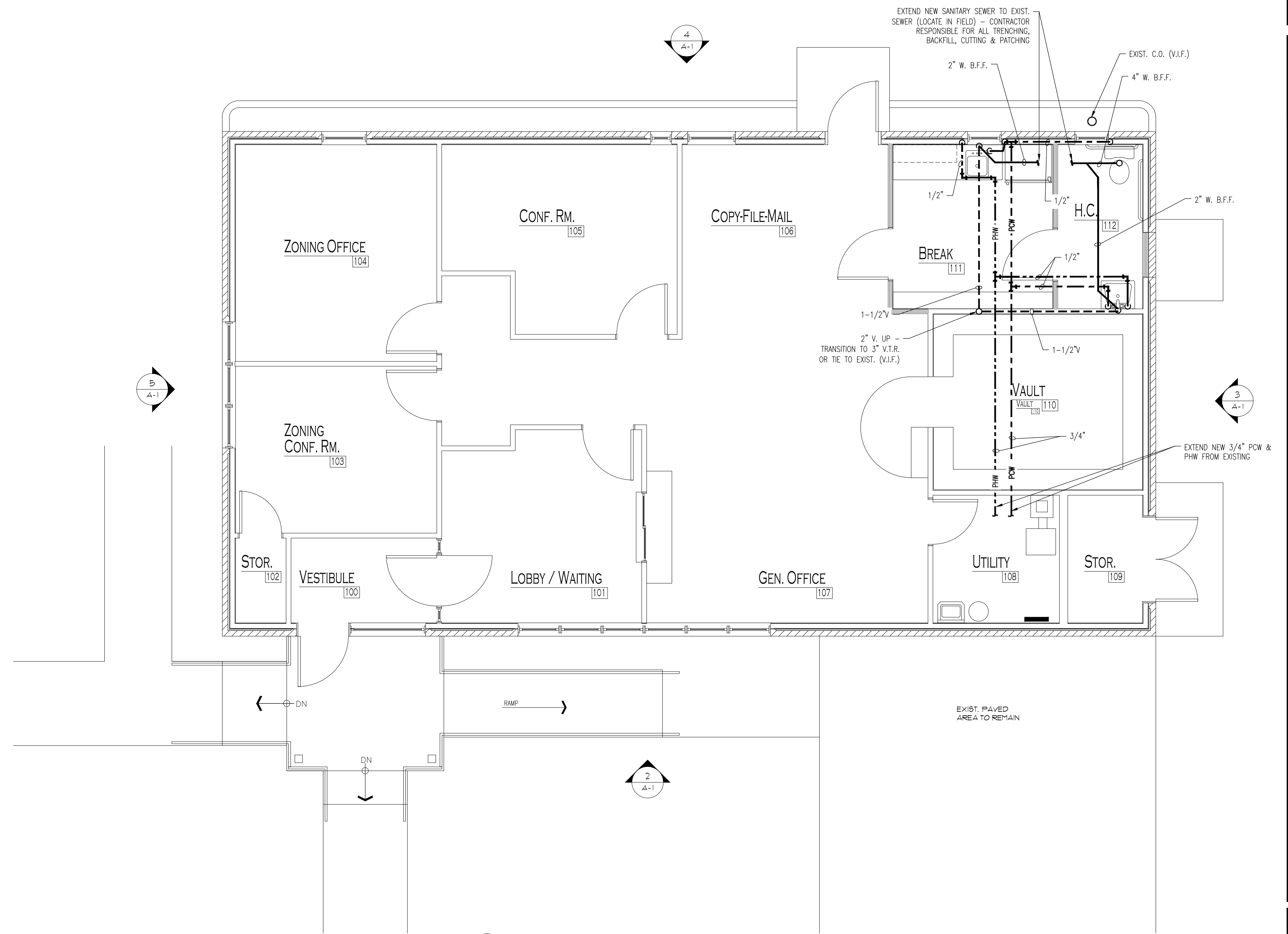
1 SANITARY & SUPPLY PLAN P-1 SCALE: 1/4"=1'-0" 0 2' 4' SCALE: 1/4"=1'-0"
