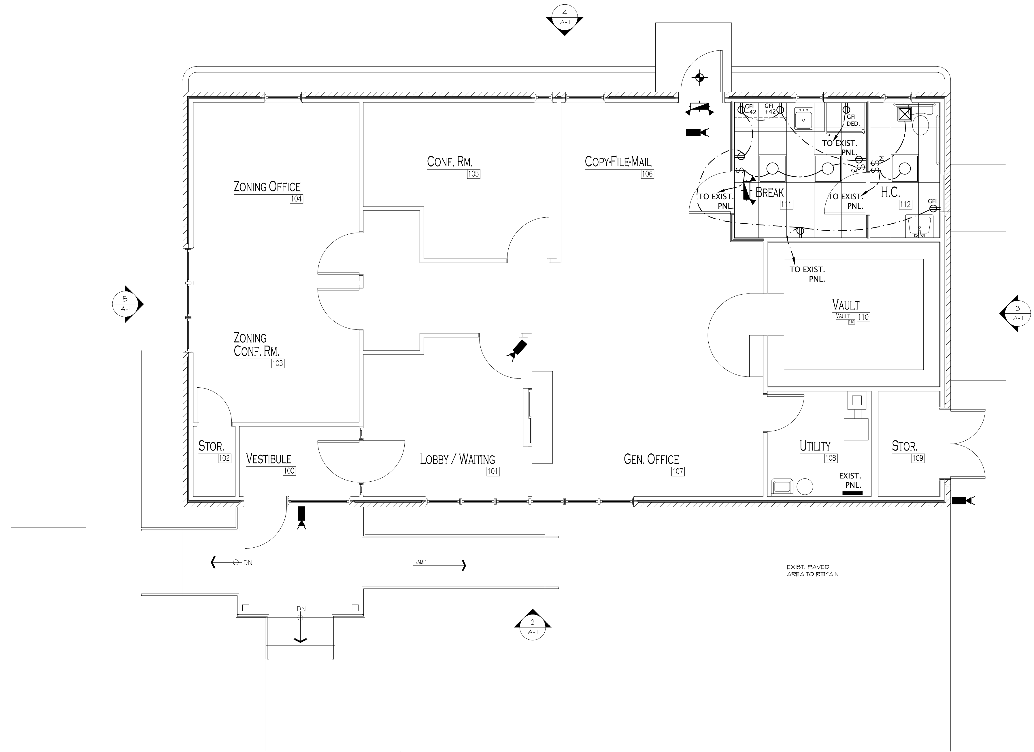
1 LIGHTING & POWER PLAN E-1 SCALE: 1/4"=1'-0"
